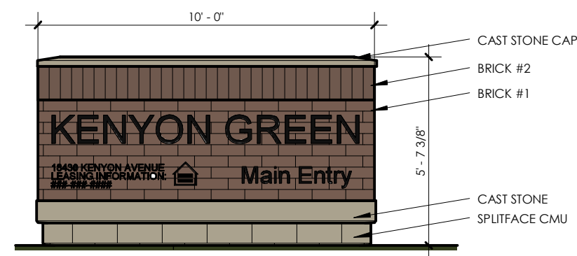
3 MONUMENT SIGN SCALE 1/4" = 1'-0"
