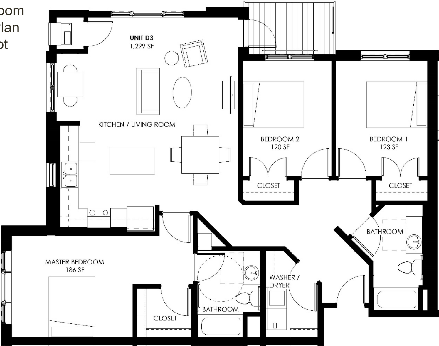
2 UNIT D3 SCALE 1/4" = 1'-0"
