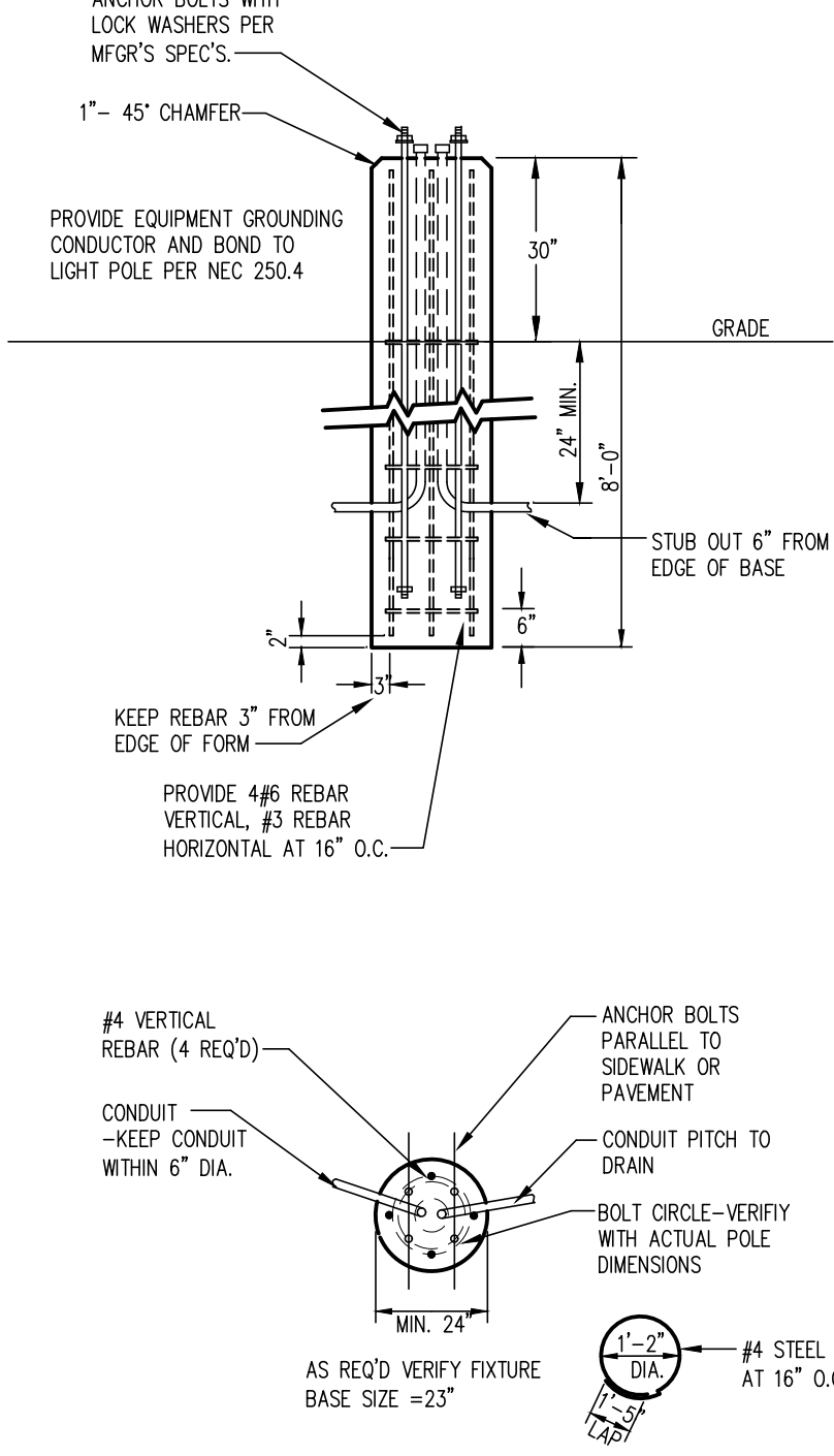
2 POLE BASE DETAIL NOT TO SCALE
