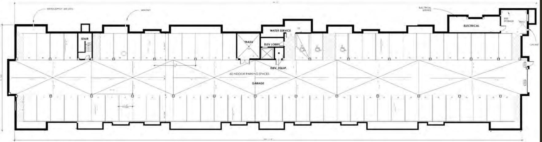
1 GARAGE PLAN SCALE: 3/32" = 1'-0"
